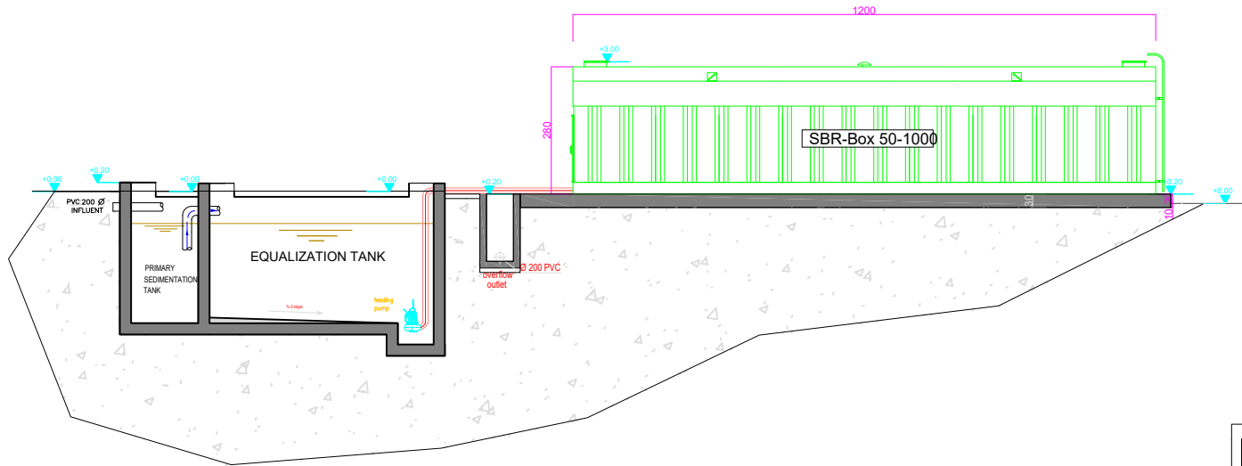
A - A CUT SECTION
